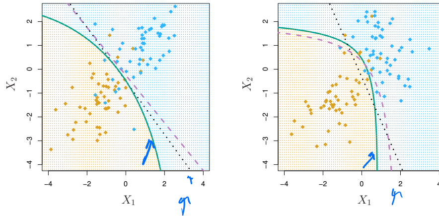
Figure 4.9 from ISL. Dashed purple curve is the Bayes classifier decision boundary. Solid green curve is QDA, dotted black line is LDA. Left: True boundary is linear. Right: True boundary is quadratic
